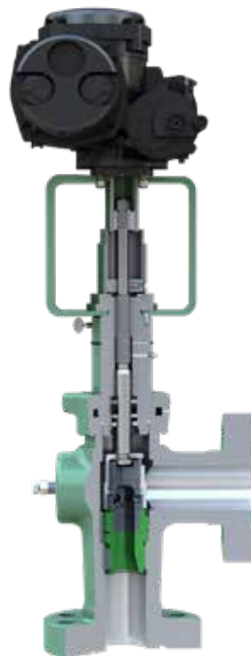
Actuated CAM30-MT choke with floating sleeve trim.
