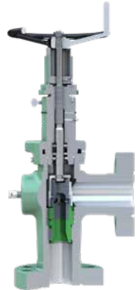
Manual CAM30-MT choke with floating sleeve trim.
