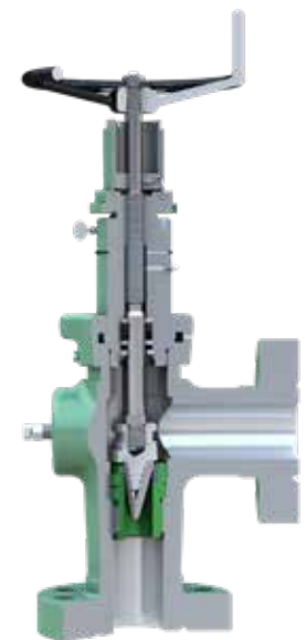
Manual CAM30-MT choke with needle-and-seat trim.
